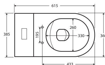
Slim Seat
