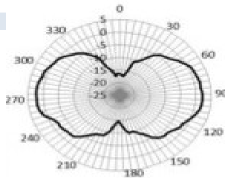
Radiation pattern 2.2- 6 GHz
