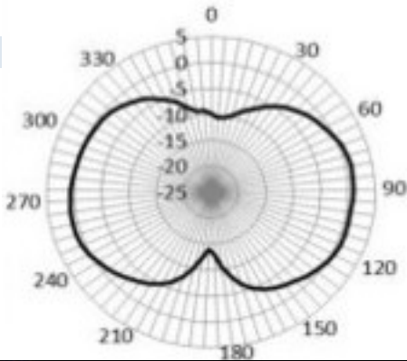
Radiation pattern 690- 960 MHz
