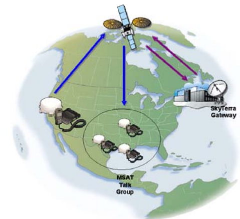
Figure 7 - Push-to-Talk Pathway
