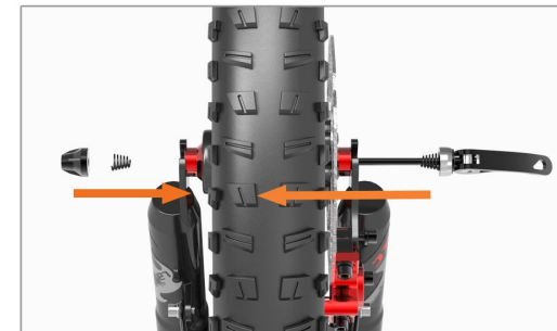
06 Insert the quick release lever from the disc brake
