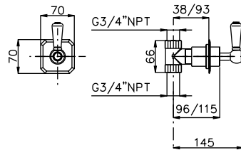
1/2" Shut Off
