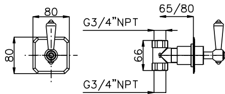
3/4" Shut Off
