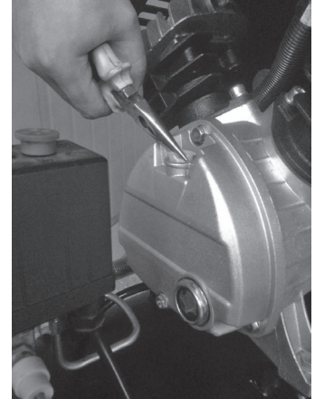
3. Locate the plastic dust plug in the oil breather hole and remove it to expose the oil breather hole.
