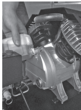
1. Always check the oil level in the pump before use. When filling, fill the oil from the oil breather hole until the oil reaches the red mark on the sight glass.
