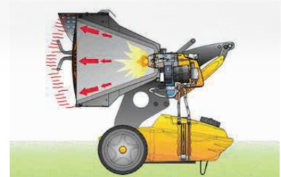
Radiant Heating - air flow
