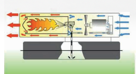
Combustion system - air flow
