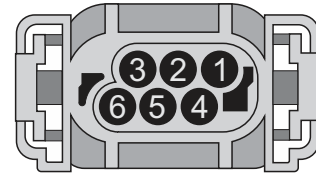
Looking into rear of plug (wire side)
