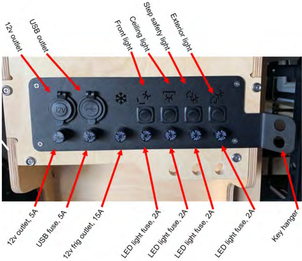
FUSE AND SWITCH PLATE AT SIDE DOOR
