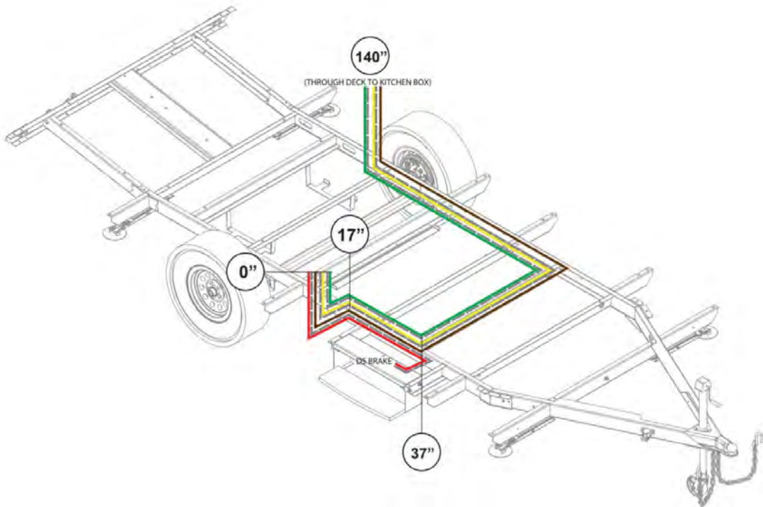
CHASSIS OVERVIEW
