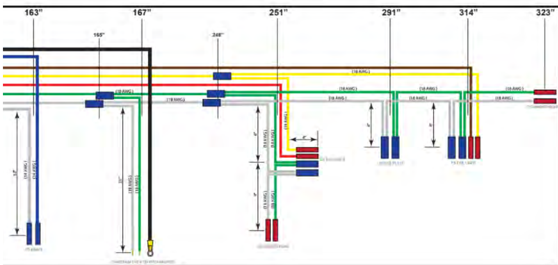
CHASSIS HARNESS
