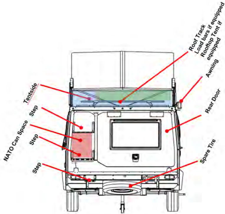
REAR ELEVATION
