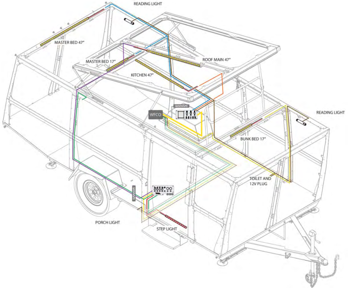
CABIN OVERVIEW
