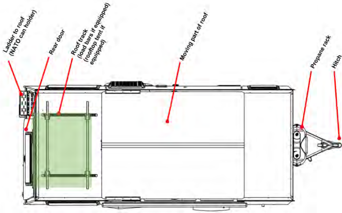
ROOF PLAN
