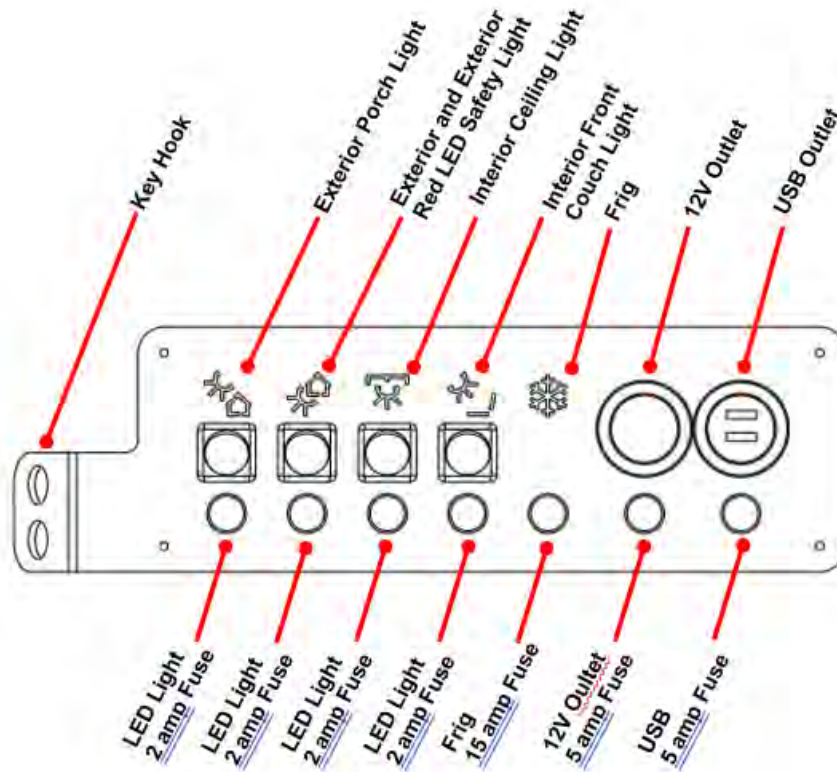
FUSE AND SWITCH PLATE AT SIDE DOOR
