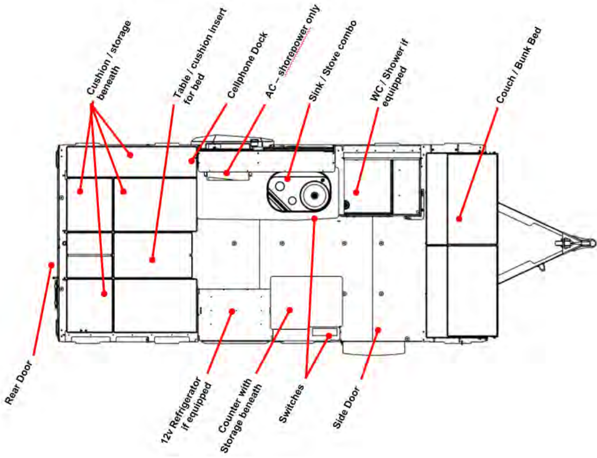
FLOOR PLAN
