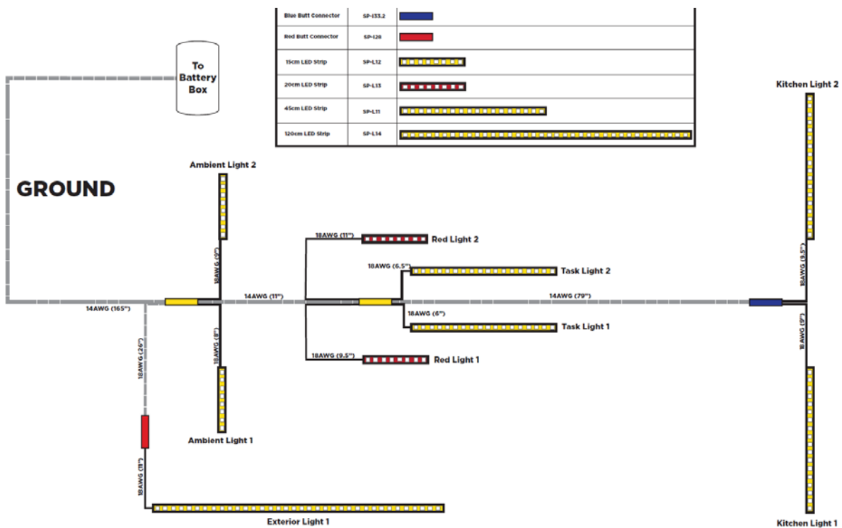
wiring diagram
