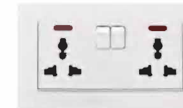
Model: PD50MSL Name: 2 Gang 3 Pin Multi-function Switched Socket With Neon Specifications: 13A 250V PCS/CTN: 60PCS/ctm
