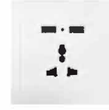
Model: D50MU2 Specifications: 13A 250V Name: Universal Socket With 2 USB PCS/CTN: 80pcs/ctn
