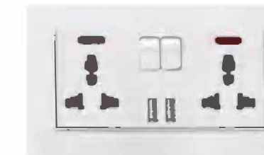
Model: PD50MSLU2 Name: 2 Gang 3 Pin Multi-function Switched Socket With Neon and USB Specifications: 13A 250V PCS/CTN: 60PCS/ctm
