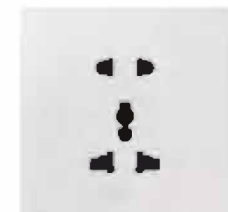
Model: D523M Specifications: 13A 250V Name: 2+3 pin Universal socket PCS/CTN: 100pcs/ctn
