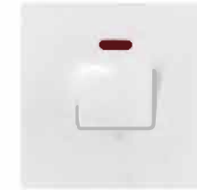
Model: D245DSL Specifications: 45A 250V Name: DP Switch With Neon PCS/CTN: 100pcs/ctn
