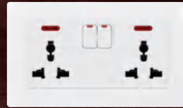
Model: PD50MSL Name: 2 Gang 3 Pin Multi-function Switched Socket With Neon Specifications: 13A 250V PCS/CTN: 60PCS/ctn
