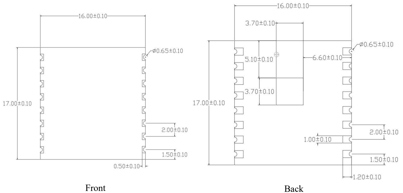
Figure 4 Dimension diagram(unit:mm)
