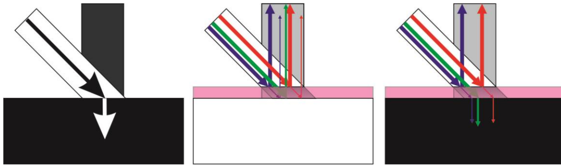
Fig 3: Measurement principle for color ink opacity measurement
