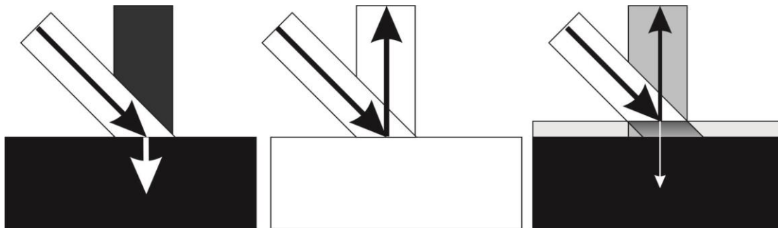
Fig 2: Measurement principle for white ink opacity measurement
