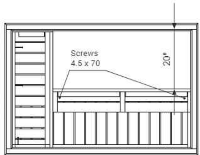
Floorplan View
