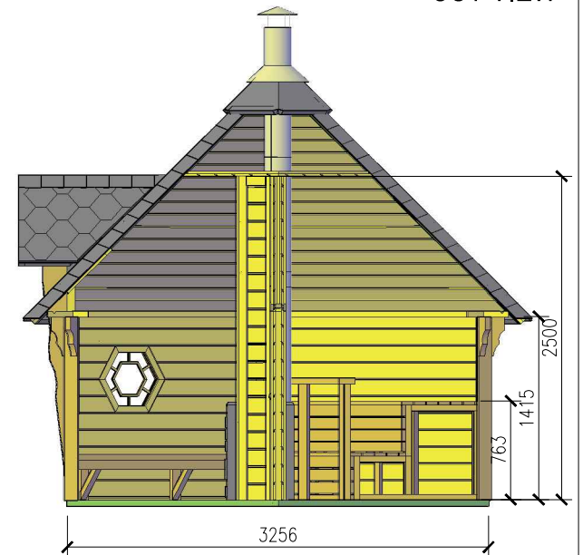
CUT VIEW
