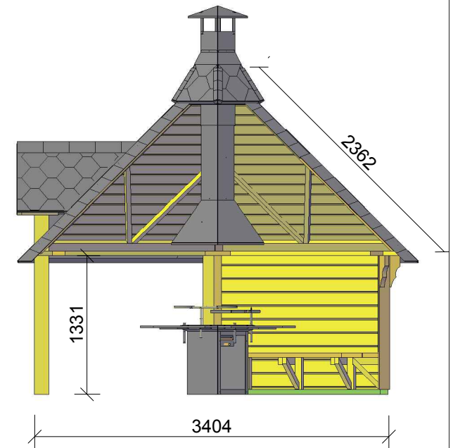
CUT VIEW
