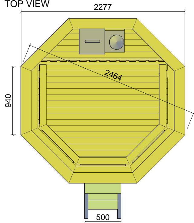
TOP VIEW
