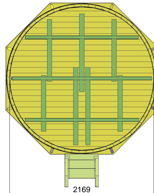
CUT VIEW
