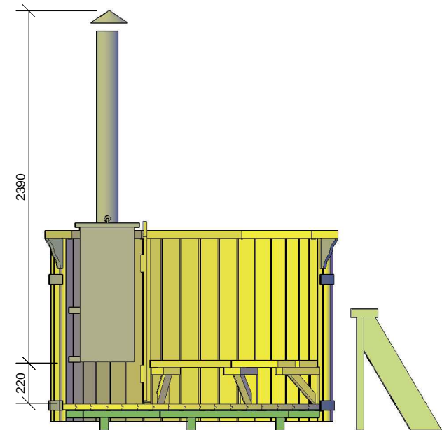
CUT VIEW
