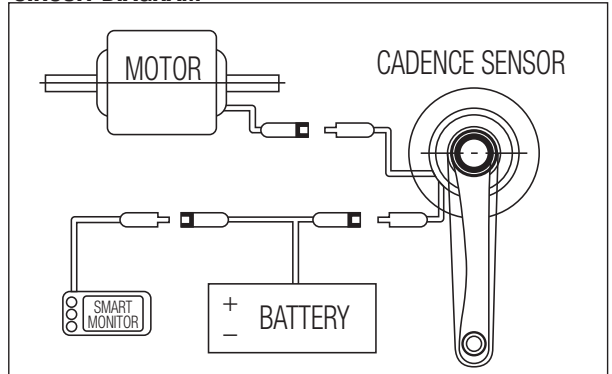
CIRCUIT DIAGRAM
