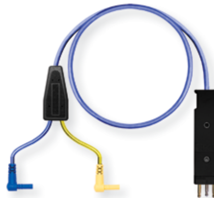
(2) R/A Shrouded Mini Banana to 463A-In Blue (6ft)
