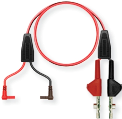
(2) R/A Shrouded Mini Banana to (2) LHTCABP Red (6ft)
