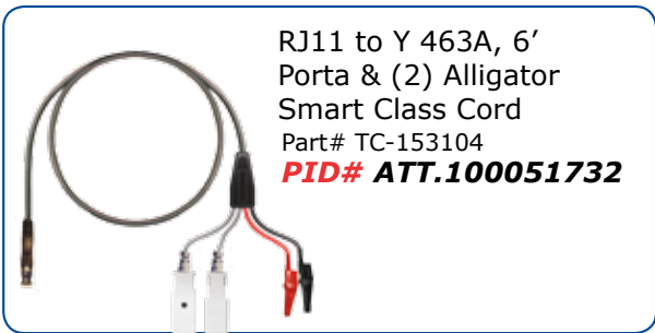
TLTS Extension Cord Part# TC-L4PEXT/30" PID# ATT.100416850
