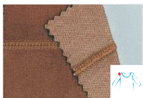
Covering stitch P21/P22
