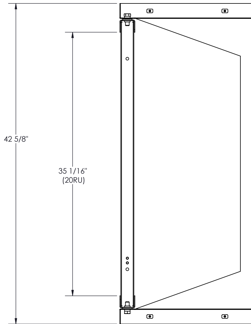
SECTION F-F
