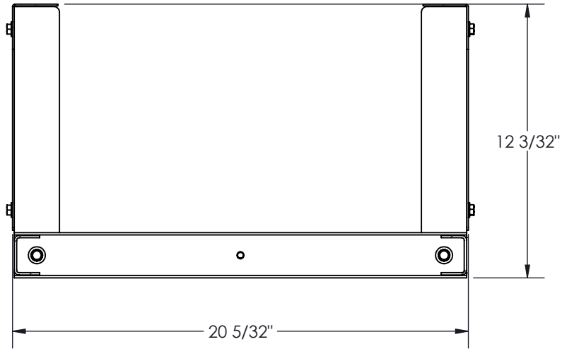
SECTION B-B
