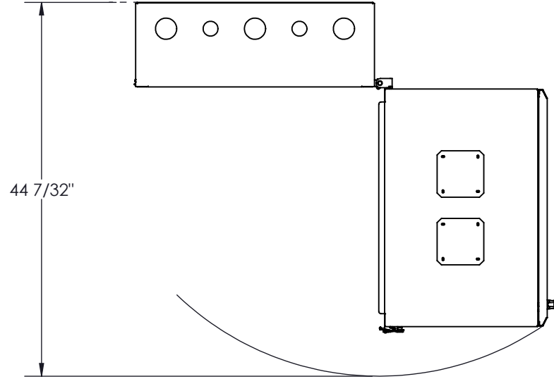
TOP VIEW REQUIRED CLEARANCE
