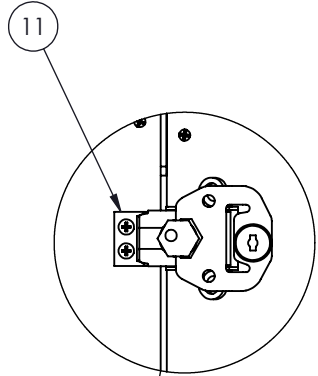
DETAIL E SCALE 1 : 4
