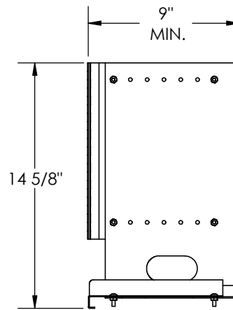
SECTION A-A 9" DEEP
