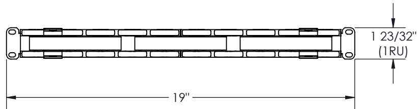
FRONT VIEW COVER NOT SHOWN
