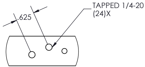
DETAIL C SCALE 1 : 2
