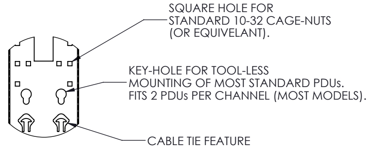
DETAIL L SCALE 1 : 8
