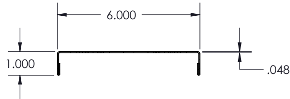
DETAIL A SCALE 1 : 4
