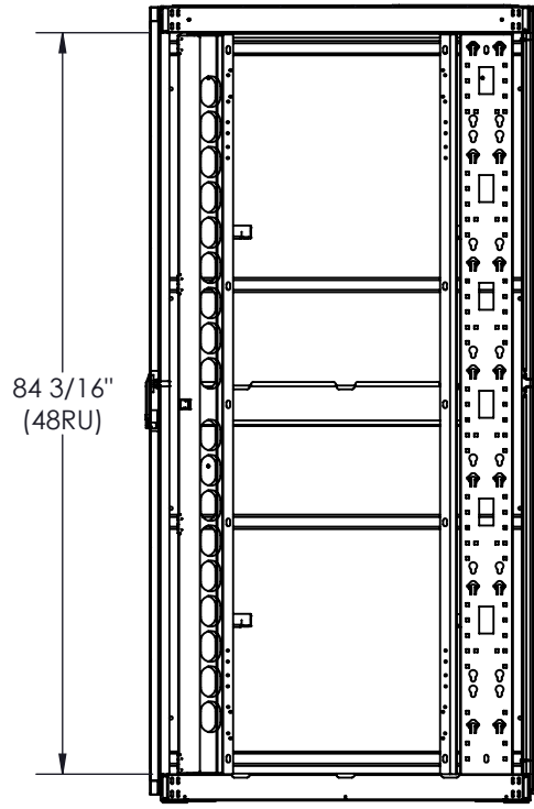
SECTION E-E
