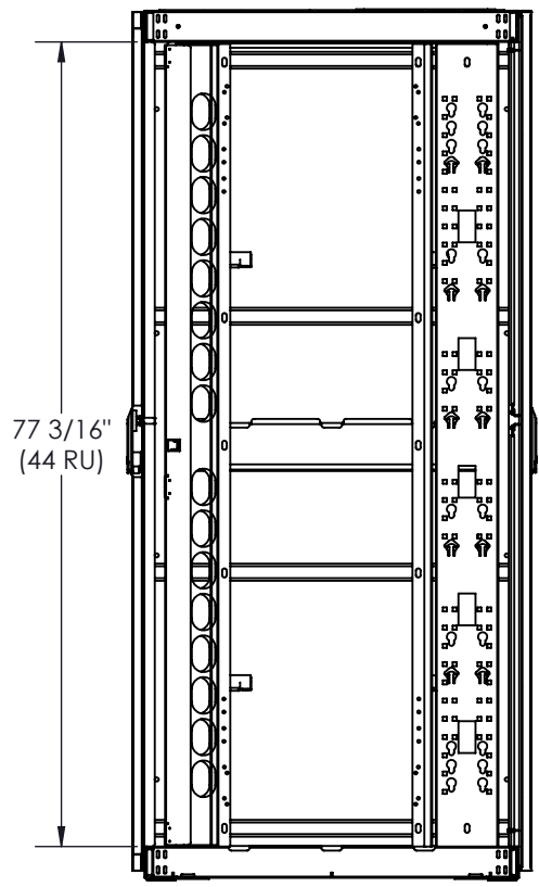
SECTION E-E
