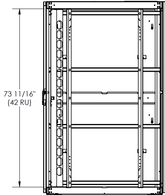
SECTION E-E
