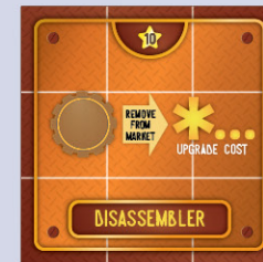
18 Large Machines
