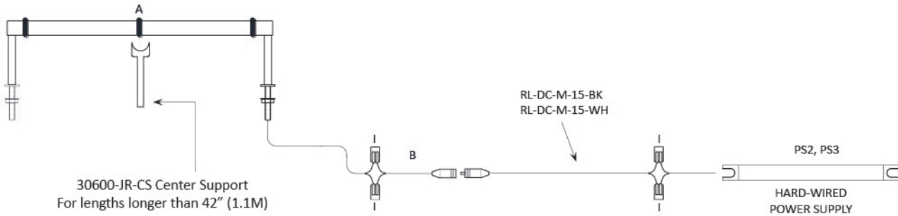
Option #2: Hardwire. Hard-Wired Wiring Diagram
