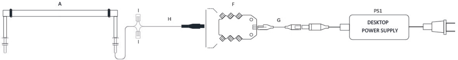
Option #1: Plug & Play. Desktop power supply Wiring Diagram [for fixtures less than 60"(152cm) long]
