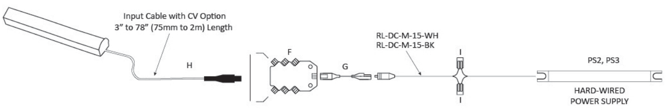
Option #1: Hardwire. Hard-Wired Wiring Diagram to constant voltage 6 port junction box
