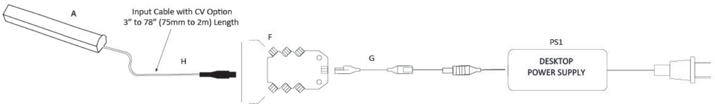
Option #1: Plug & Play to constant voltage 6 port junction box. Desktop power supply Wiring Diagram
