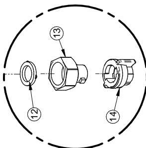
DETAIL E
