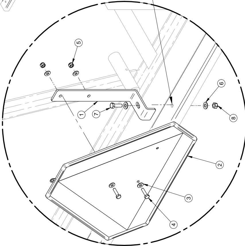
DETAIL A 1:5.56
