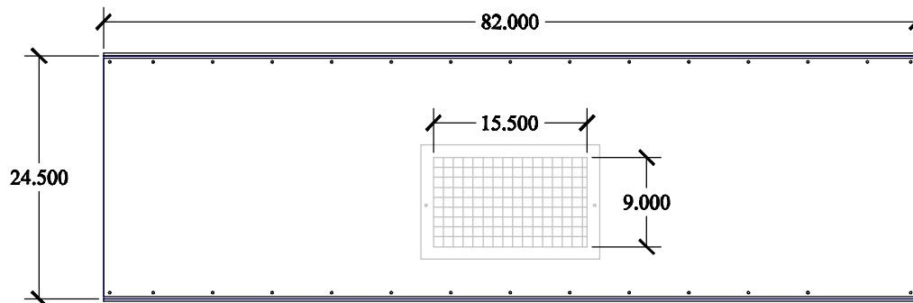
FRONT VIEW, EXHAUST
