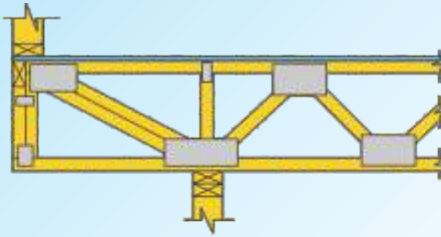
Cantilever with an exterior wall on the end.
