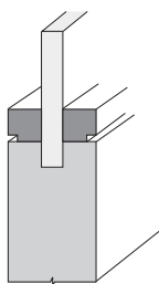
Optional quirk bead
