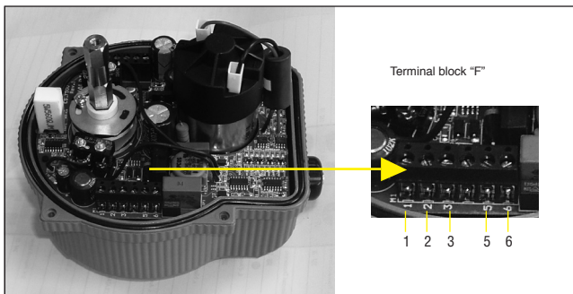
Fig.3 Plate of supply 100-240V AC and particular of terminal block "F"
