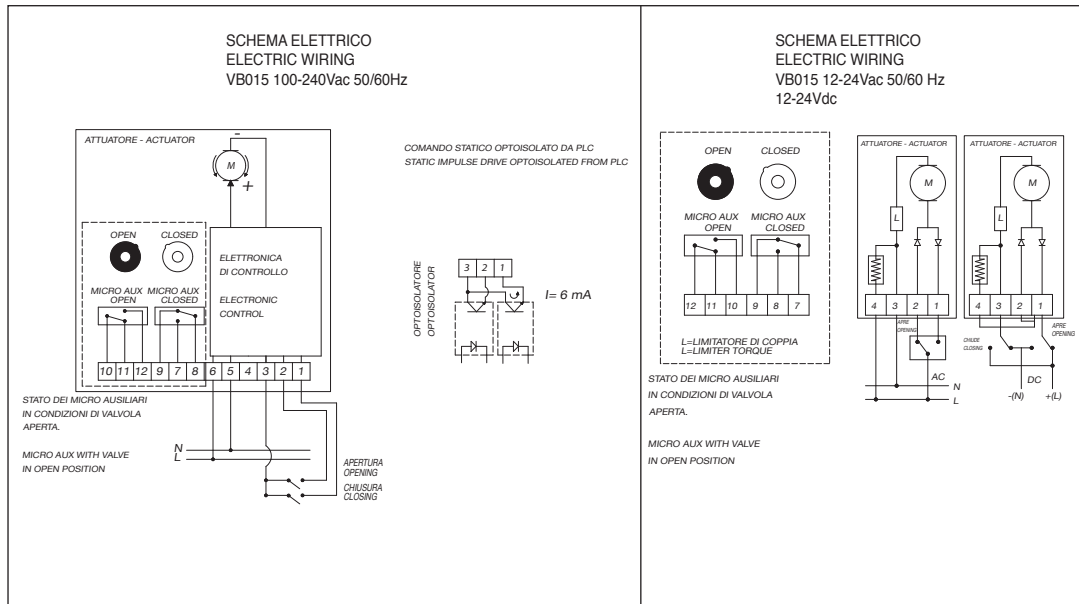
Fig. 5 Electric wiring diagram to cable the actuators
