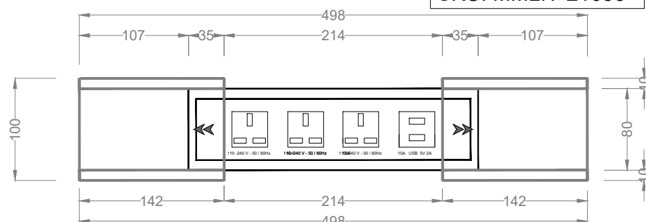
TOP VIEW - DOOR OPEN
