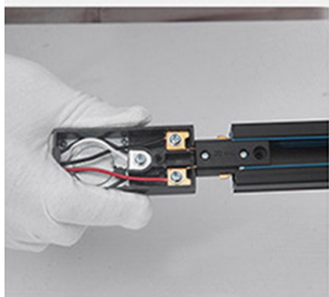
4. Insert the junction box into the track
