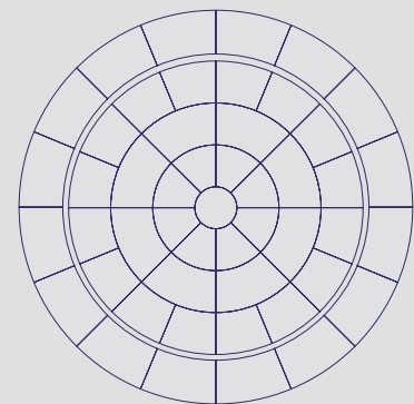
3600mm DIAMETER CIRCLE EXTENSION KIT
