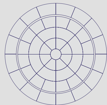
3600mm DIAMETER CIRCLE EXTENSION KIT
