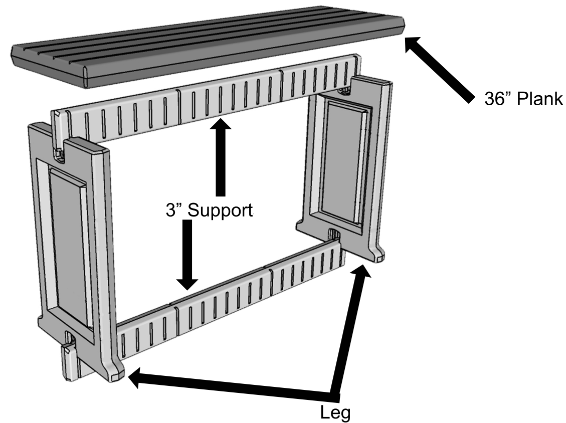
Exploded Labeled Diagram
