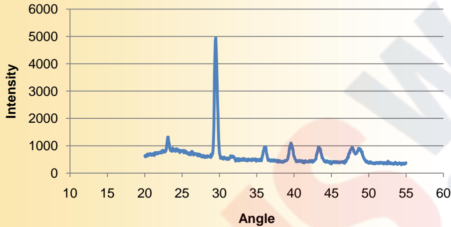
XRD Untreated
